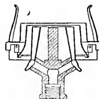
Fig. 3157. BURNER FOR No. 1 VESTIBULE LAMP.
